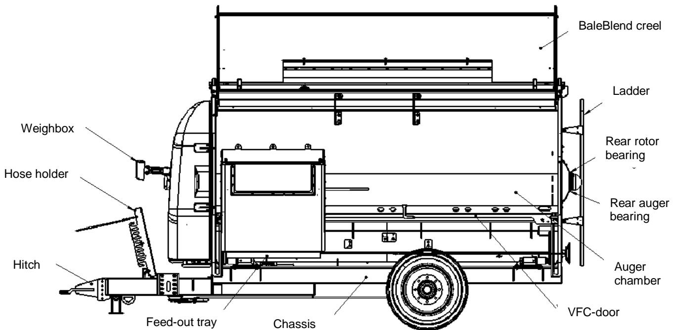
Figure 1: KEENAN MechFiber320 mixer wagon (BaleBlend option shown)
