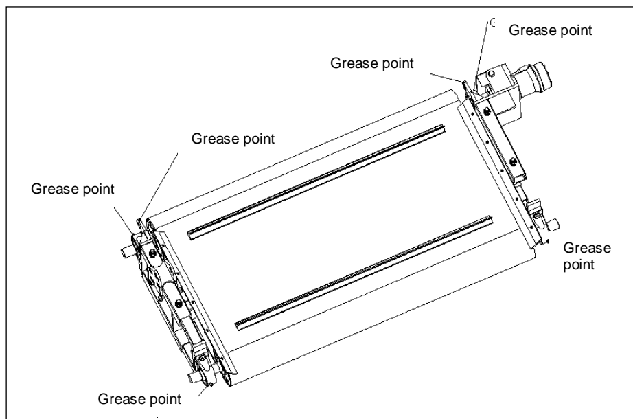
Figure 19: Side elevator greasing points
