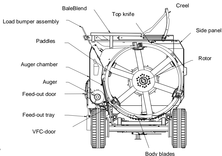
Figure 2: KEENAN MechFiber rear view
