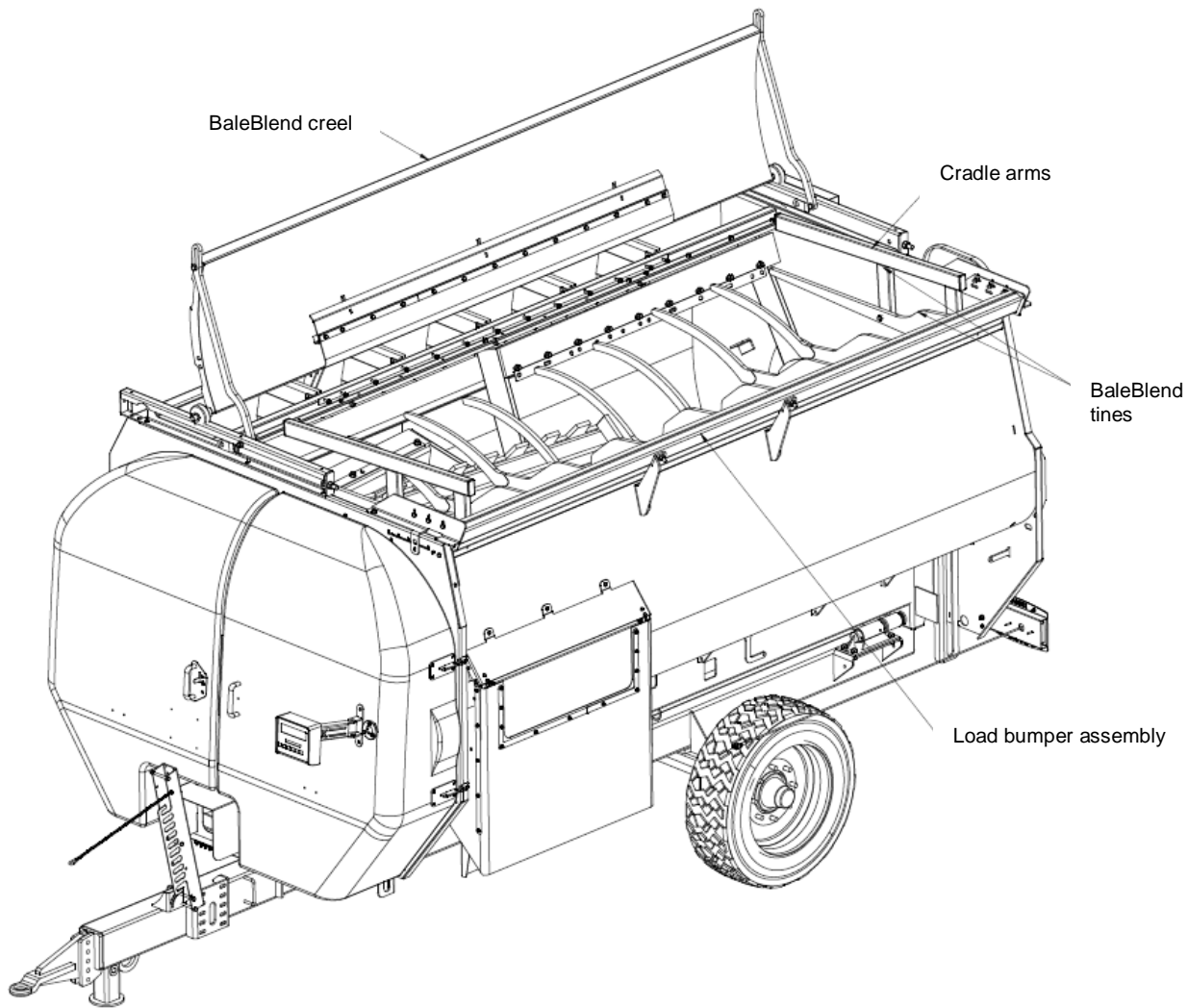
Figure 17: MechFiber machine with BaleBlend attachment
