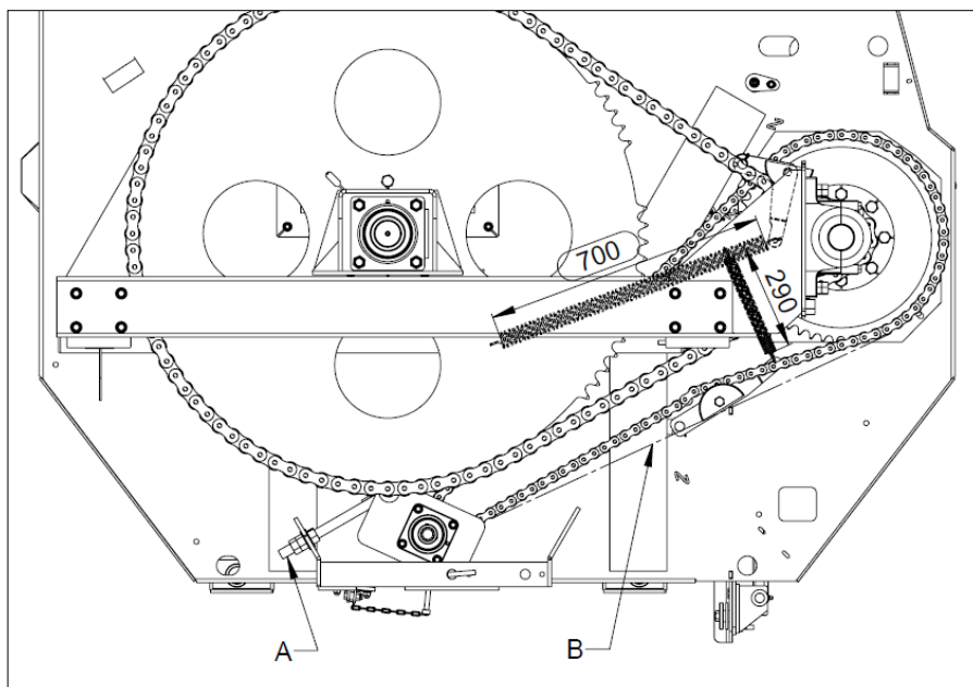
Figure 11: MechFiber270 and 320 chain tensioning (showing springs fully stretched)
