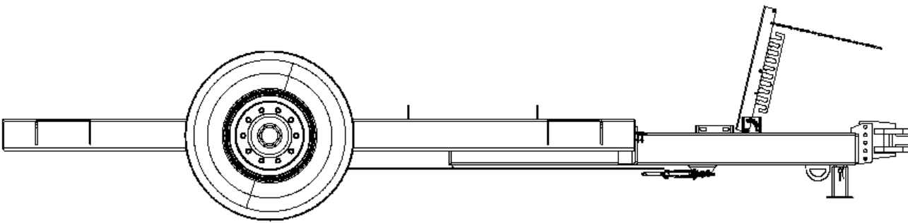
Figure 6.3: Clevis hitch (typically for the U.S. market)
